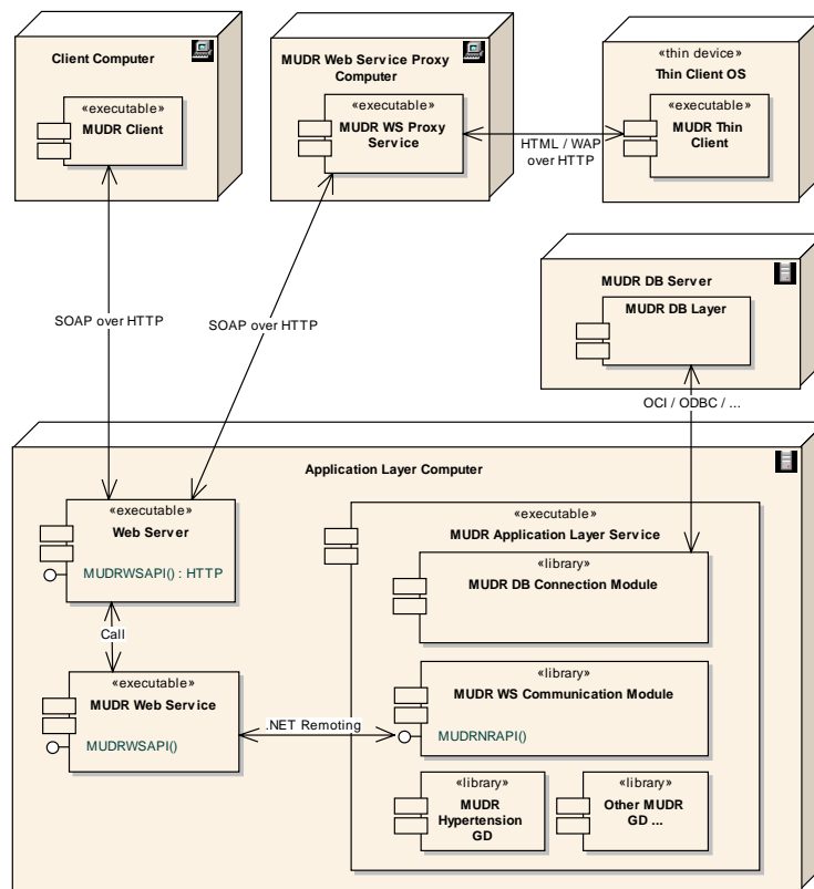
Fig. 3. MUDR II Extended Architecture.
