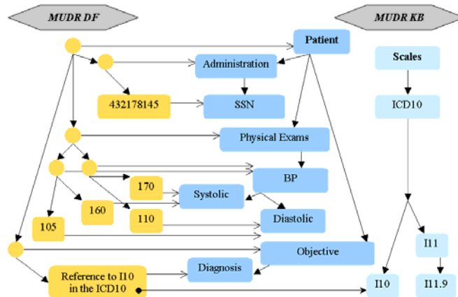
Fig. 1. Fragment of the MUDR Information Storage Model.
